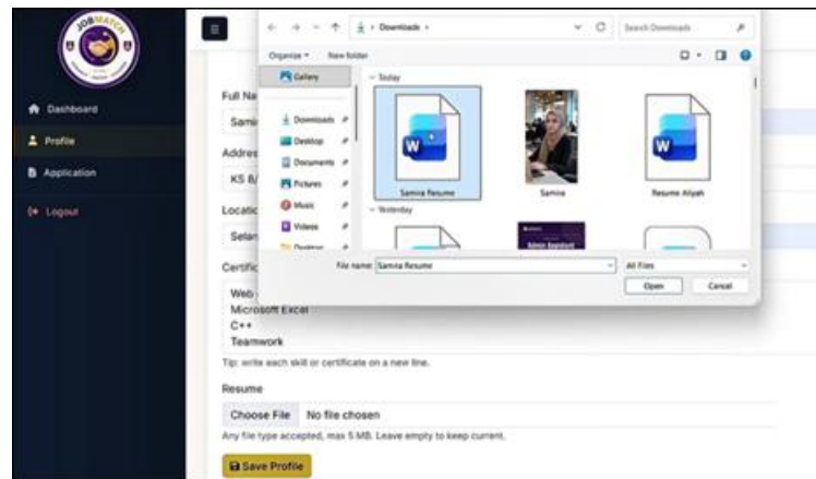
Figure 9: Resume Upload
