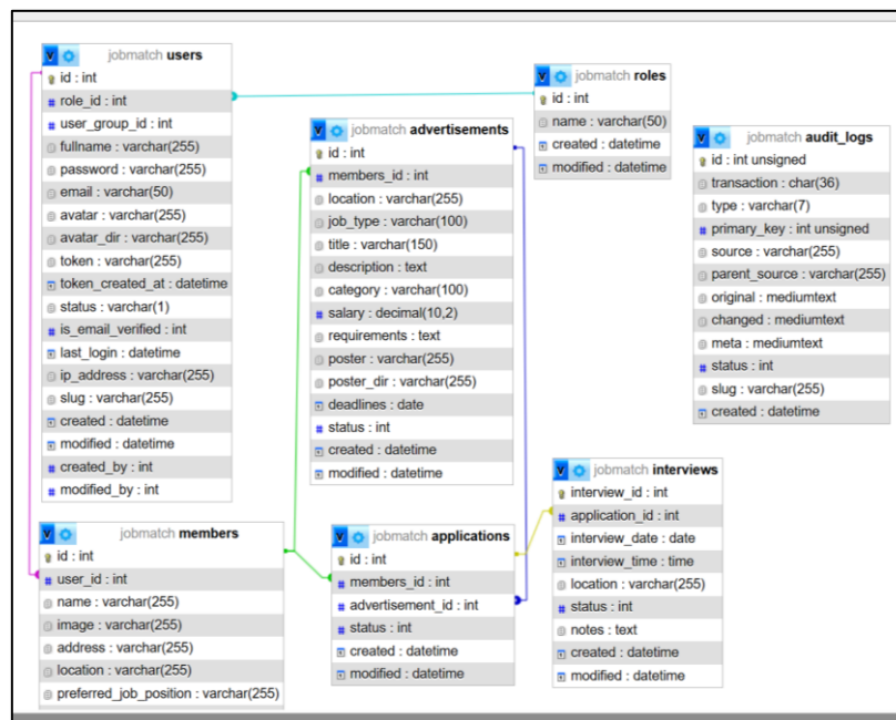
Figure 1: JobMatch's ERD
