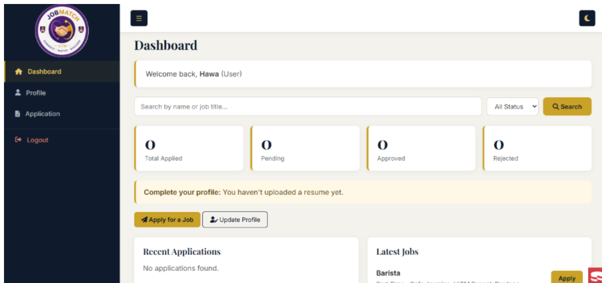
Figure 2: Layout JobMatch
