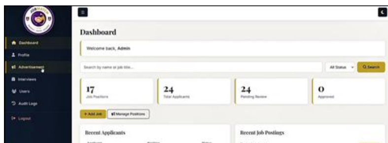
Figure 10:Admin Dashboard
